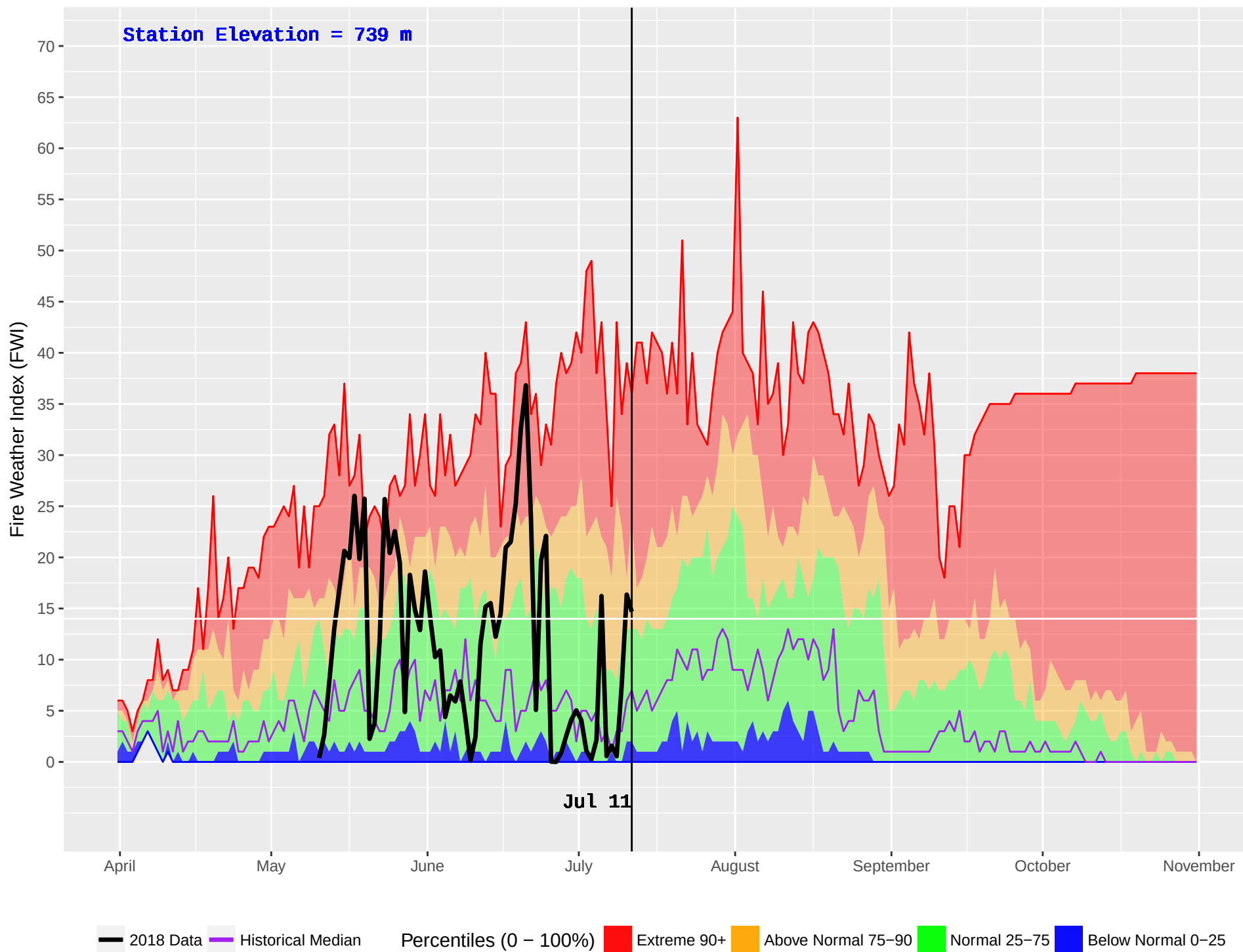
BEAR LAKE (149) : Historical (1980–2016) and Current (2018) Noon Fire Weather Index (FWI)
