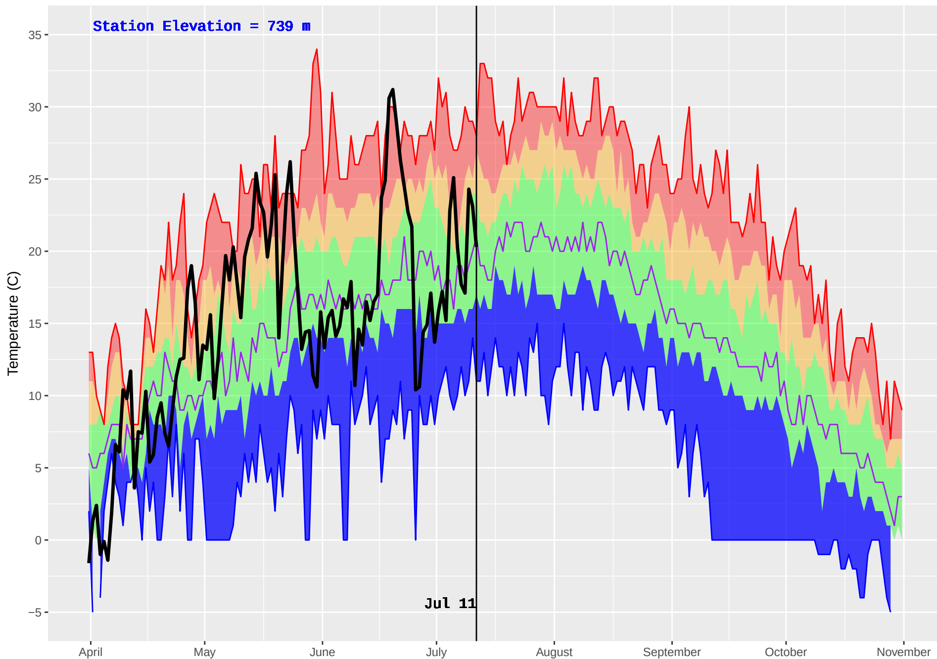
BEAR LAKE (149) : Historical (1980–2016) and Current (2018) Noon Temperature
