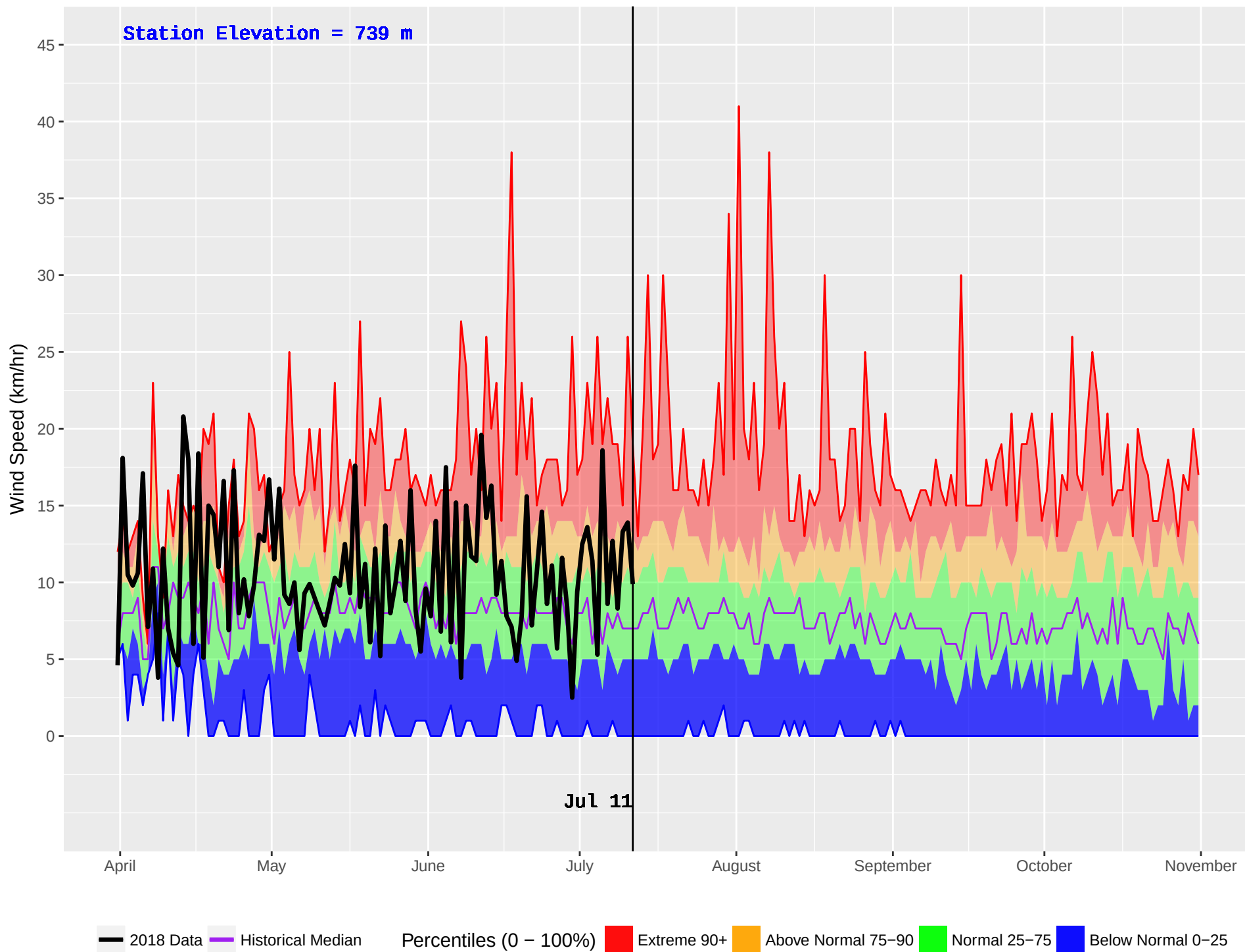
BEAR LAKE (149) : Historical (1980–2016) and Current (2018) Noon Wind Speed
