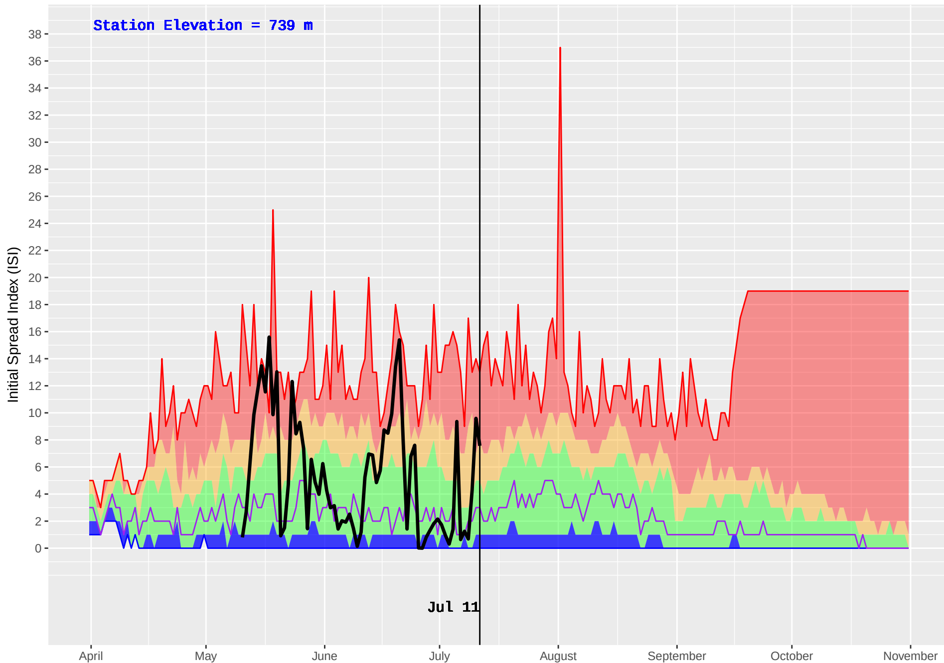
BEAR LAKE (149) : Historical (1980–2016) and Current (2018) Noon Initial Spread Index (ISI)
