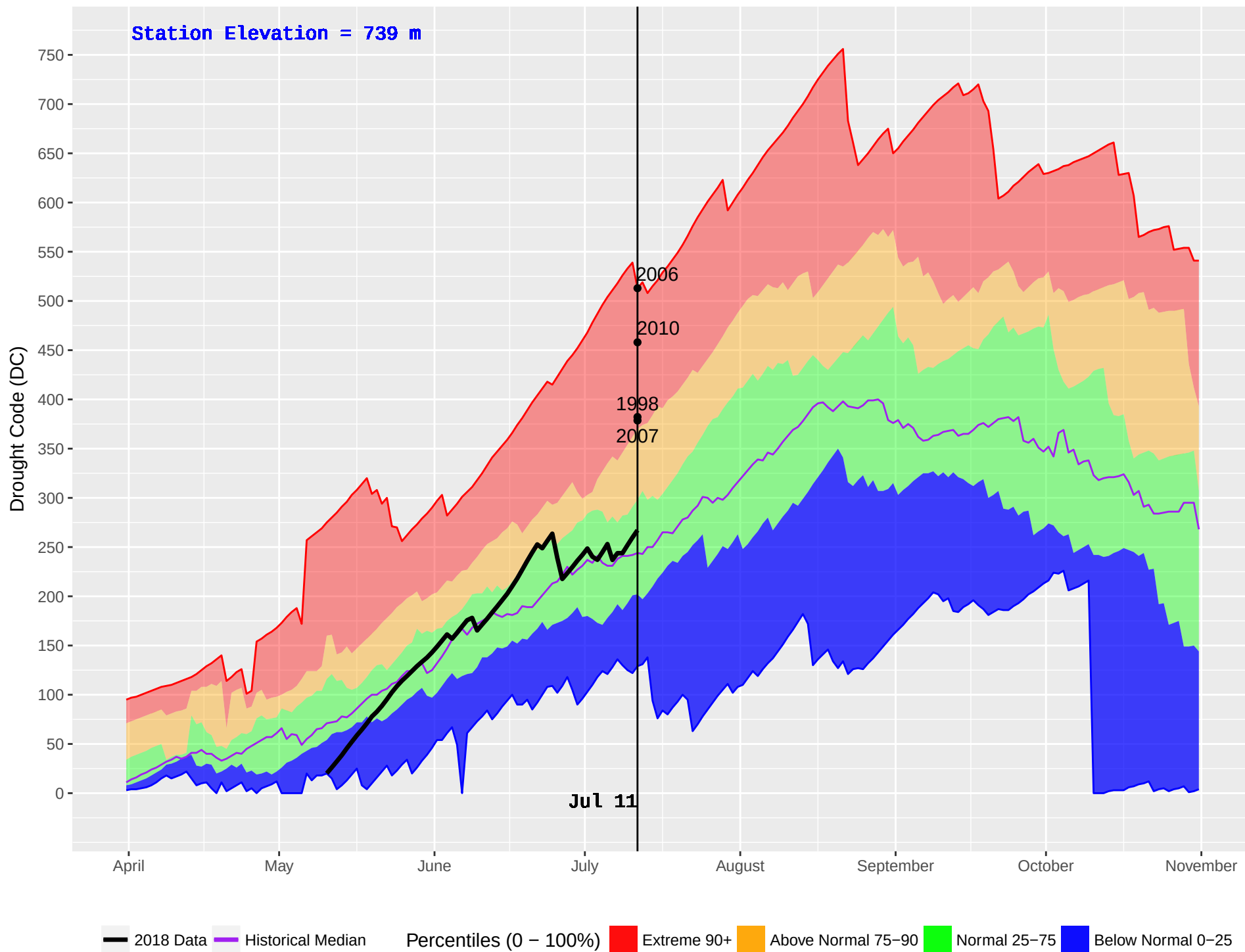
BEAR LAKE (149) : Historical (1980–2016) and Current (2018) Noon Drought Code (DC)
