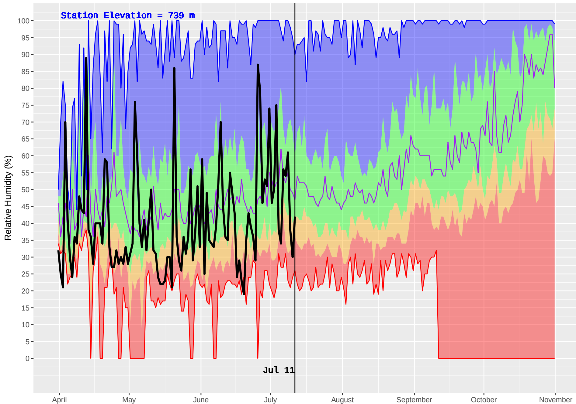
BEAR LAKE (149) : Historical (1980–2016) and Current (2018) Noon Relative Humidity
