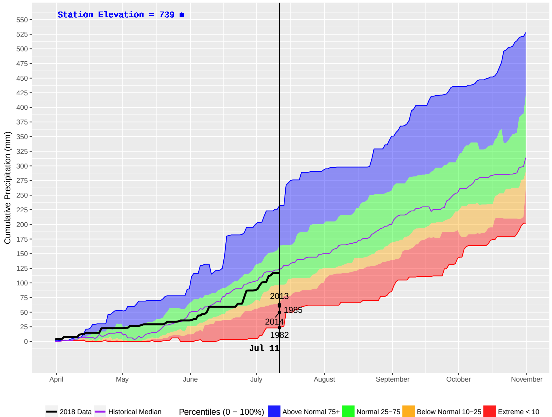
BEAR LAKE (149) : Historical (1980–2016) and Current (2018) Noon Cumulative Precipitation
